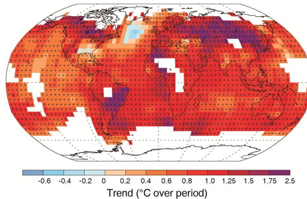
(b) Observed change in average surface temperature 1901–2012
